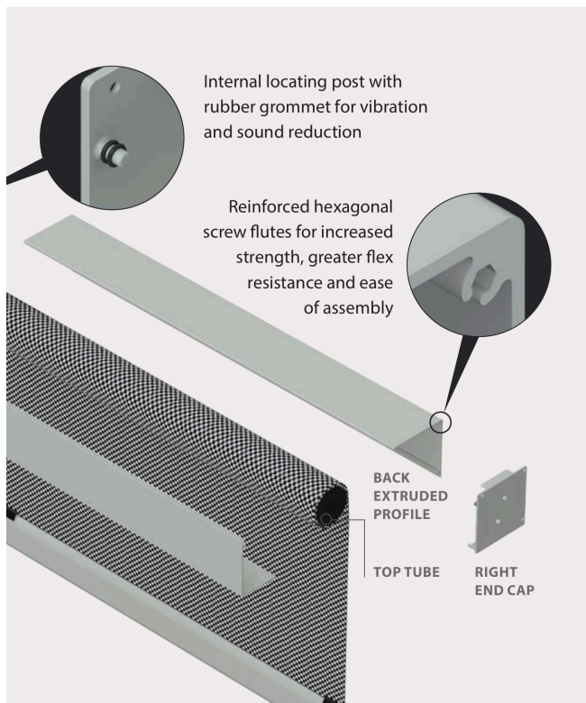
Cutaway of a track-blind headbox & bottom rail. Profiles may vary.
